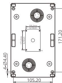
JHAS80-EL80R
