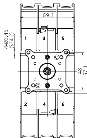
JHAS80-PM125R-3
