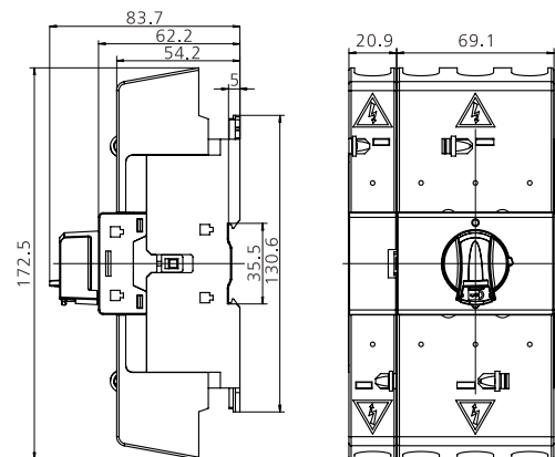
JHAS80-DB100R-4 JHAS80-DB125R-4
