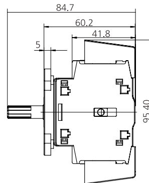
JHAS80-PM16R-4 JHAS80-PM25R-4
