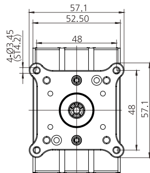
JHAS80-PM80R-3
