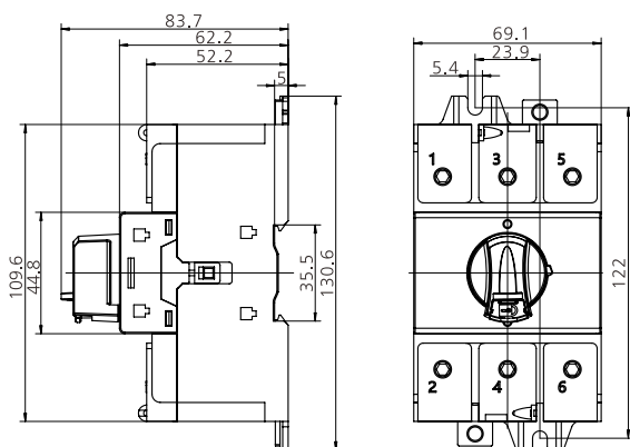
JHAS80-DB100R-3 JHAS80-DB125R-3
