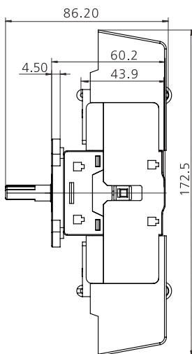
JHAS80-PM100R-3
