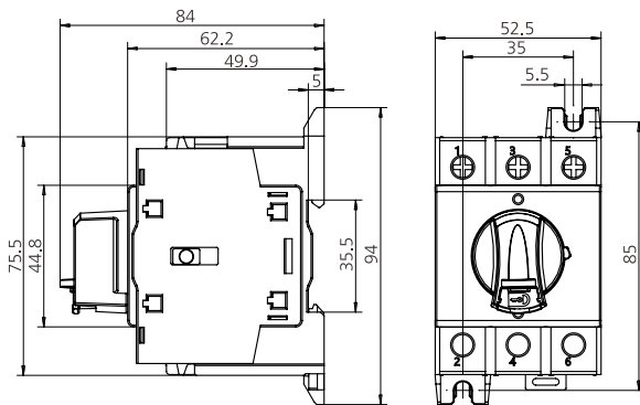
JHAS80-DB63R-3 JHAS80-DB80R-3
