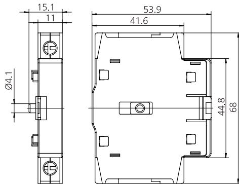
JHAS80-PS40 JHAS80-PN40 JHAS80-PD40 JHAS80-PE40
