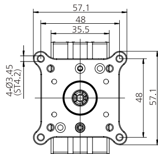
JHAS80-PM32R-3 JHAS80-PM40R-3
