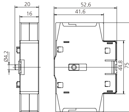
JHAS80-PS80R JHAS80-PN80R JHAS80-PD80R JHAS80-PE80R
