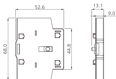
JHAS80-P1R JHAS80-P2R
