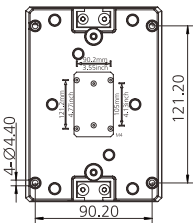
JHAS80-ELA40R
