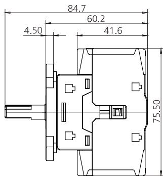
JHAS80-PM63R-3
