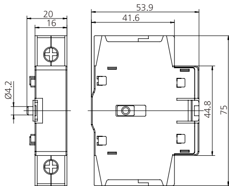
JHAS80-PS80 JHAS80-PN80 JHAS80-PD80 JHAS80-PE80
