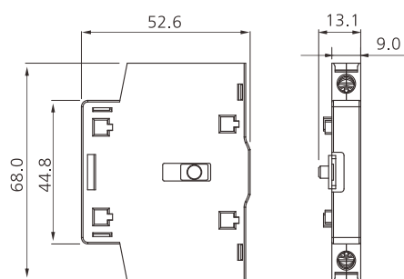
JHAS80-P1 JHAS80-P2
