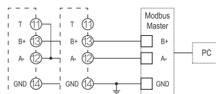
Rs485 Modbus communication port
