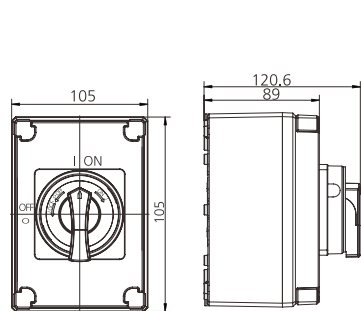
Overall and Installation Dimension(mm)
