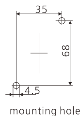
mounting hole
