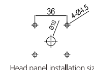
Head panel installation size
