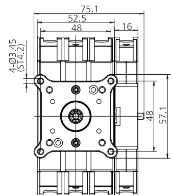
JHAS80-PM80R-4
