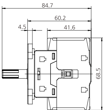
JHAS80-PM16R-3 JHAS80-PM25R-3
