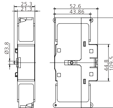
JHAS80-PSR125 JHAS80-PNR125 JHAS80-PSR125 JHAS80-PER125
