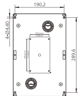
JHAS80-EL125R
