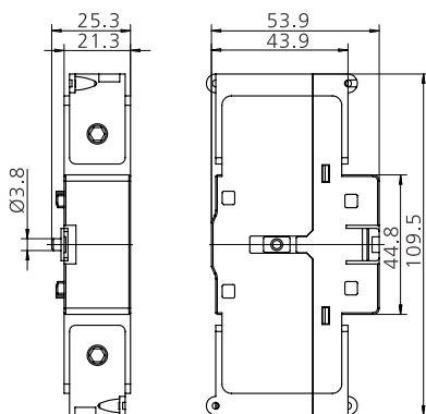
JHAS80-PS125 JHAS80-PN125 JHAS80-PS125 JHAS80-PE125
