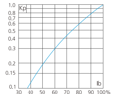
Power Losses
