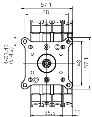
JHAS80-PM32R-4 JHAS80-PM40R-4
