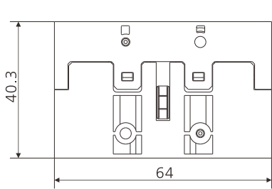
JHAC69-ACC01/02
