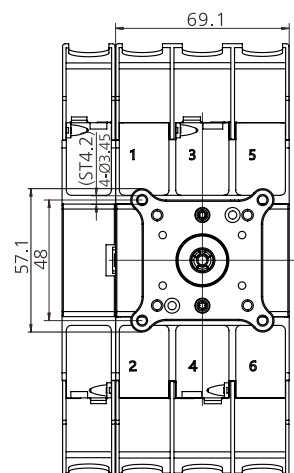
JHAS80-PM125R-4
