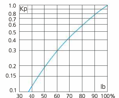
Power Losses
